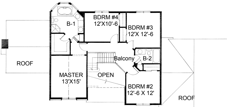
SECOND FLOOR 1046 S.F.
