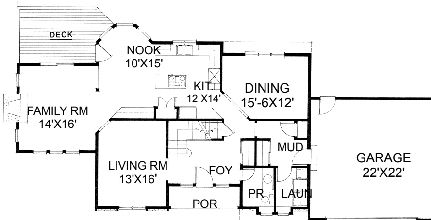
FIRST FLOOR 1294 S.F.
