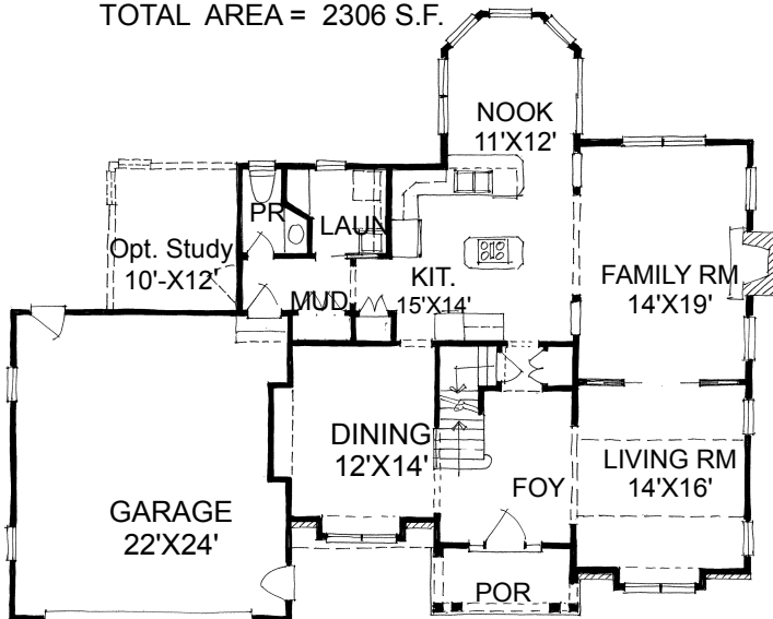
FIRST FLOOR 1310 S.F.
