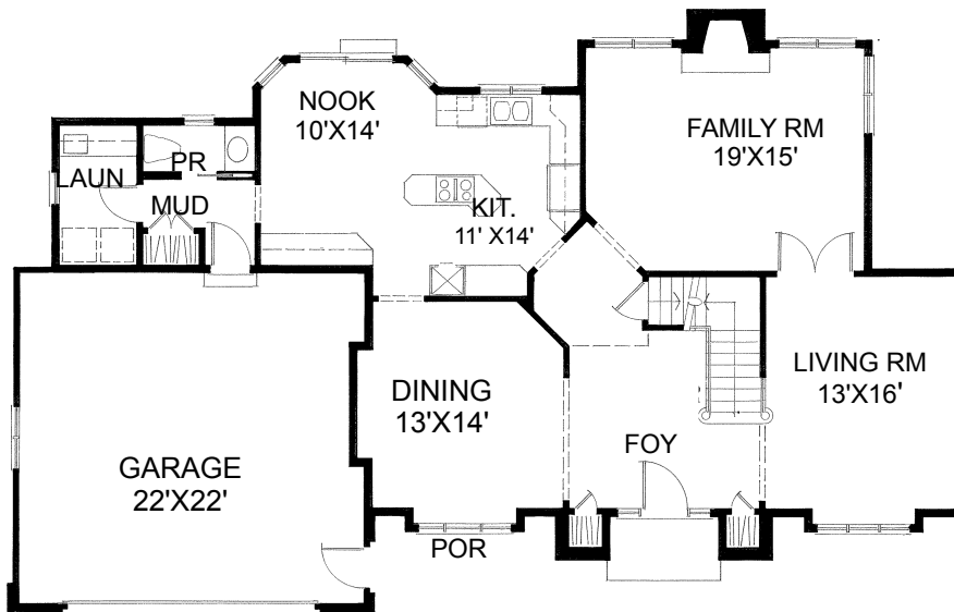
FIRST FLOOR 1327 S.F.
