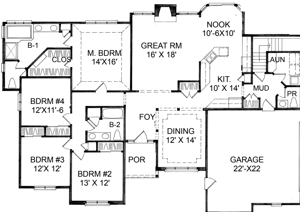
FLOOR PLAN AREA: 2289 S.F.
