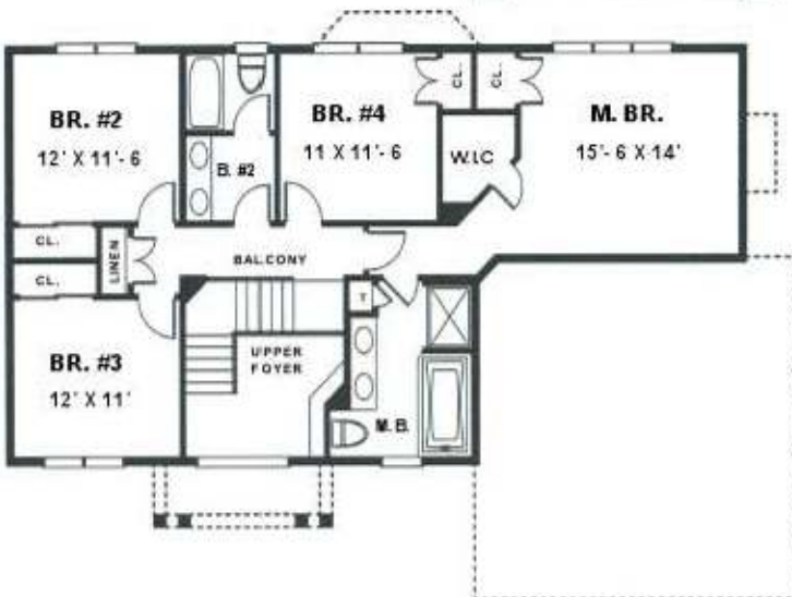
SECOND FLOOR AREA: 1000 SQ. FT.
