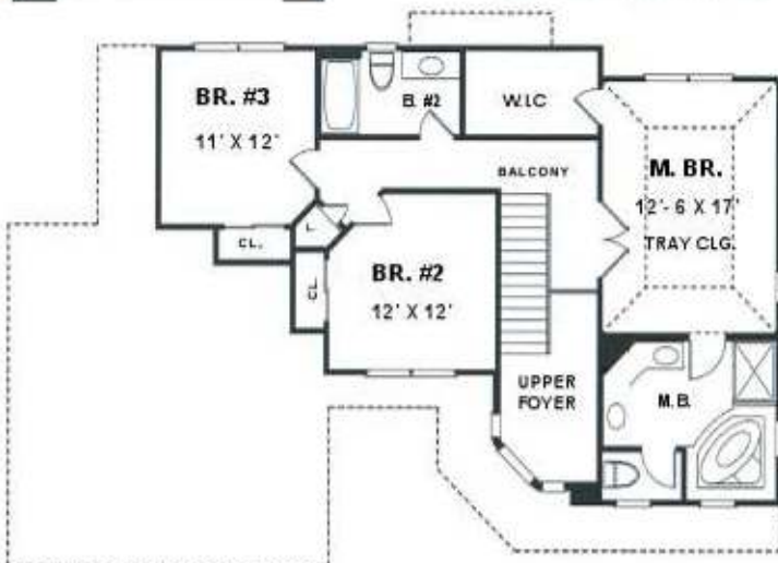
SECOND FLOOR AREA: 870 SQ. FT.
