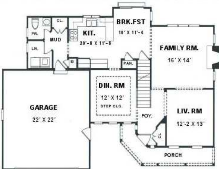
FIRST FLOOR AREA: 1021 SQ. FT.
