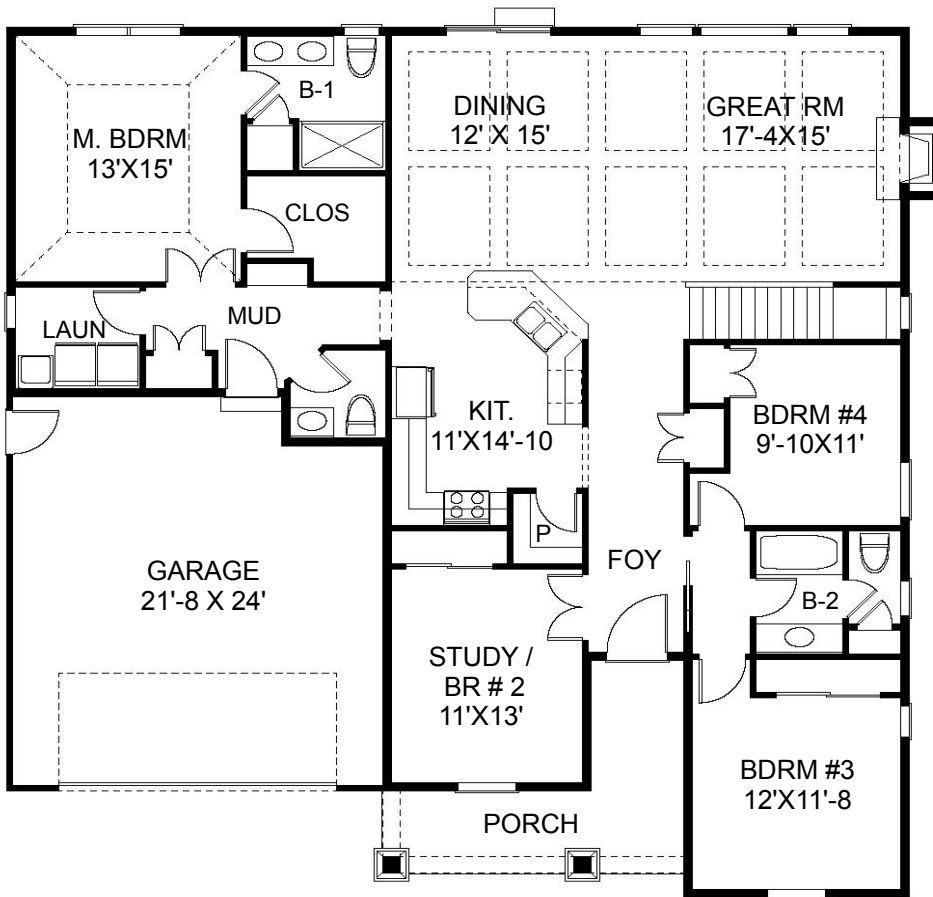
FLOOR PLAN AREA: 1958 S.F.
