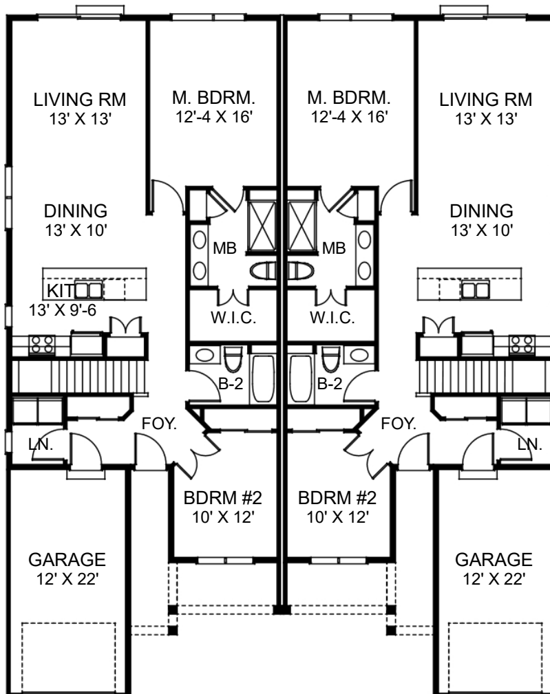
FLOOR PLAN 1271 S.F.
