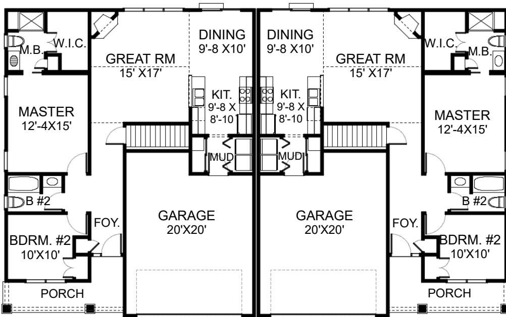
FLOOR PLAN 1245 S.F.
